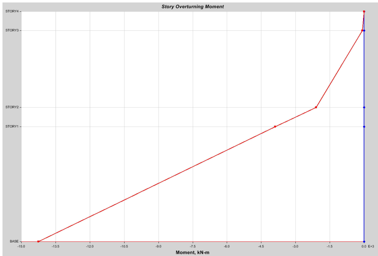
Moment de rasturnare seism x
