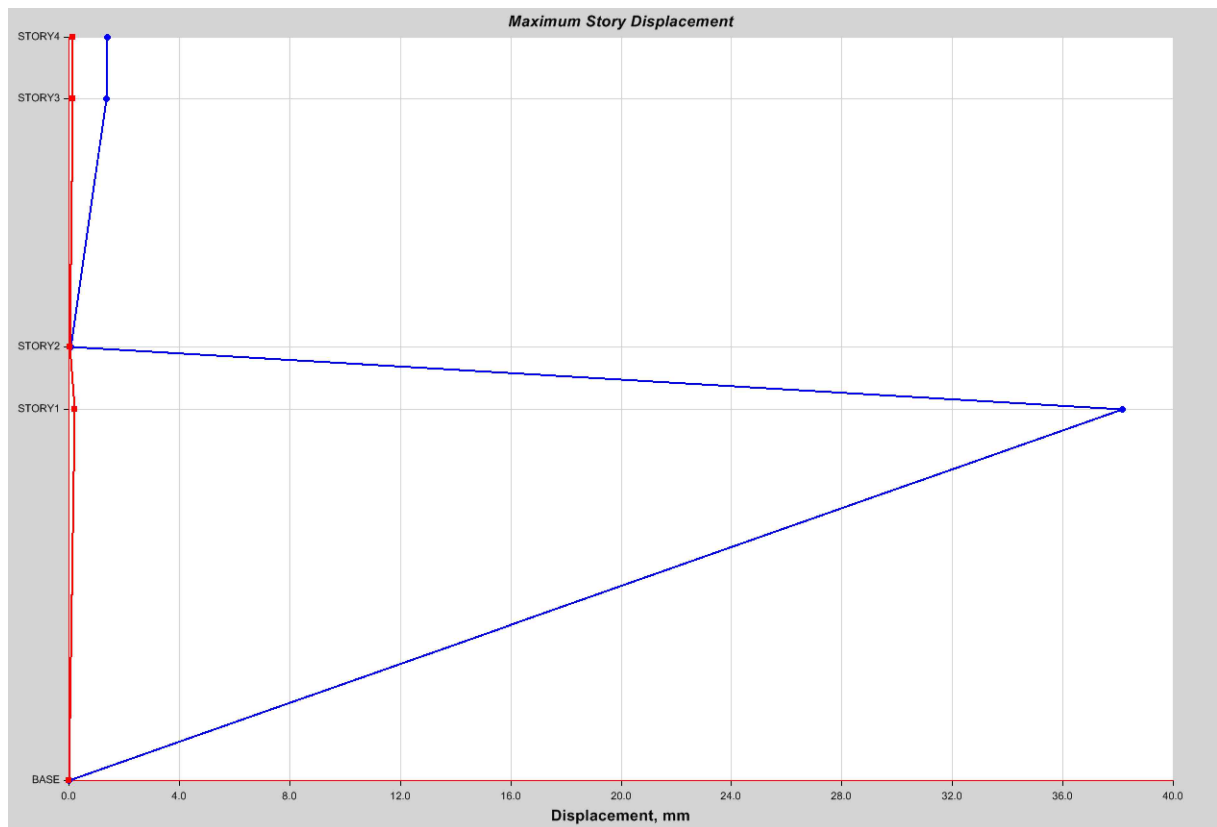
Deformatii absolute seism x
